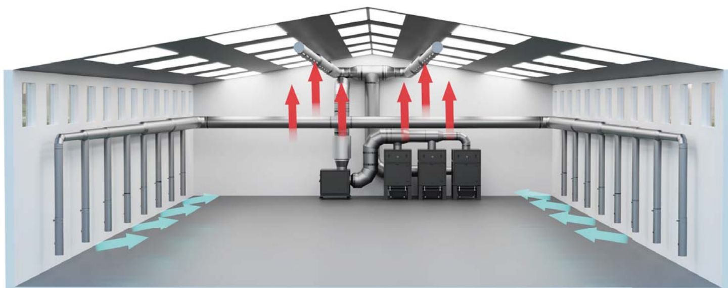
Installation example: Layered ventilation system in a hall
