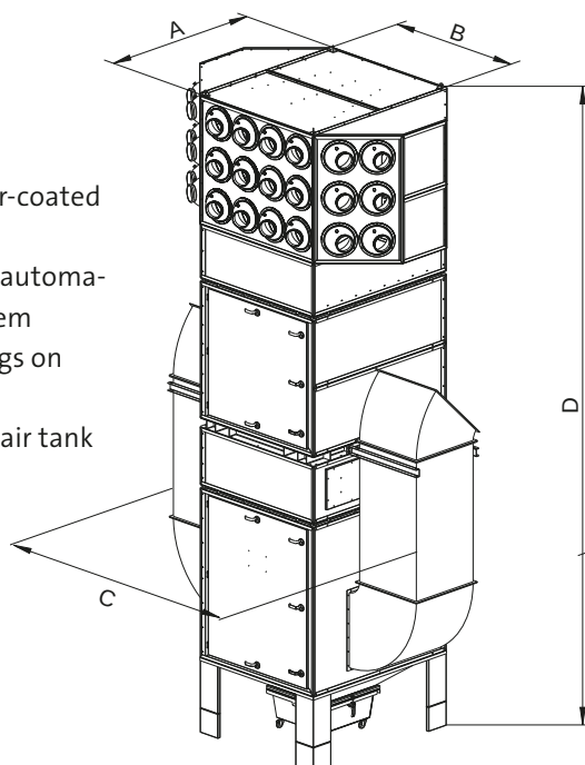
Unit with silencer housing
