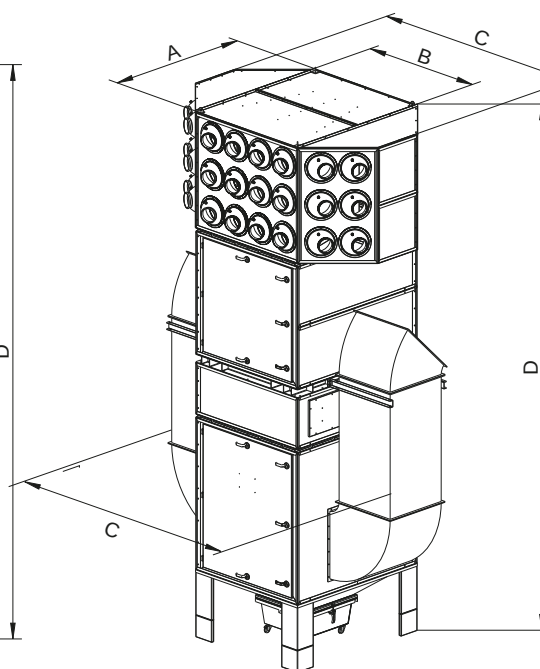
Unit without silencer housing
